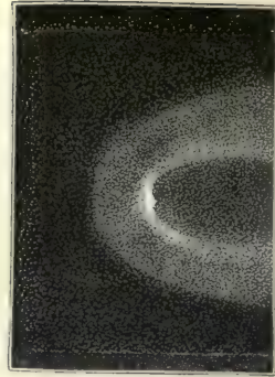
October 12. (Pepe.)
